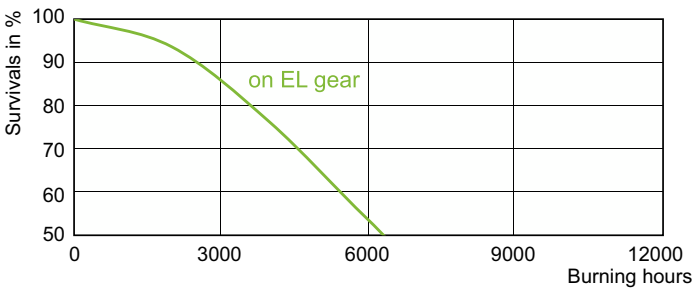
Life Expectancy Diagram - MASTER CDM-T 250W/830 G12 1CT/12
