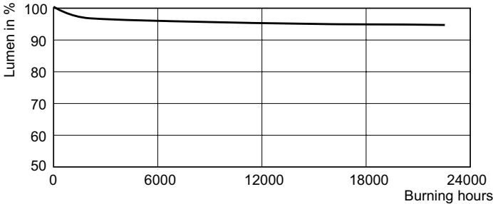
Lumen Maintenance Diagram - MASTER SOX-E PSG 36W BY22d T50 1SL/12
