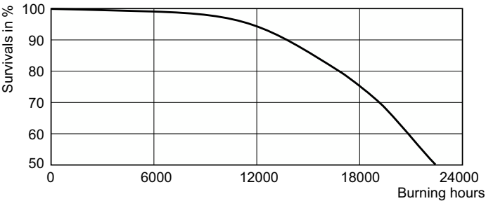
Life Expectancy Diagram - MASTER SOX-E PSG 36W BY22d T50 1SL/12
