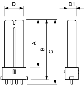
PL-S 9W/108/4P
