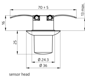
sensor head
