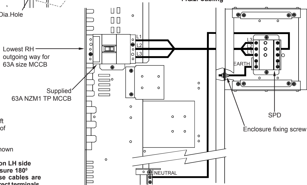
FIG.2. Cabling
