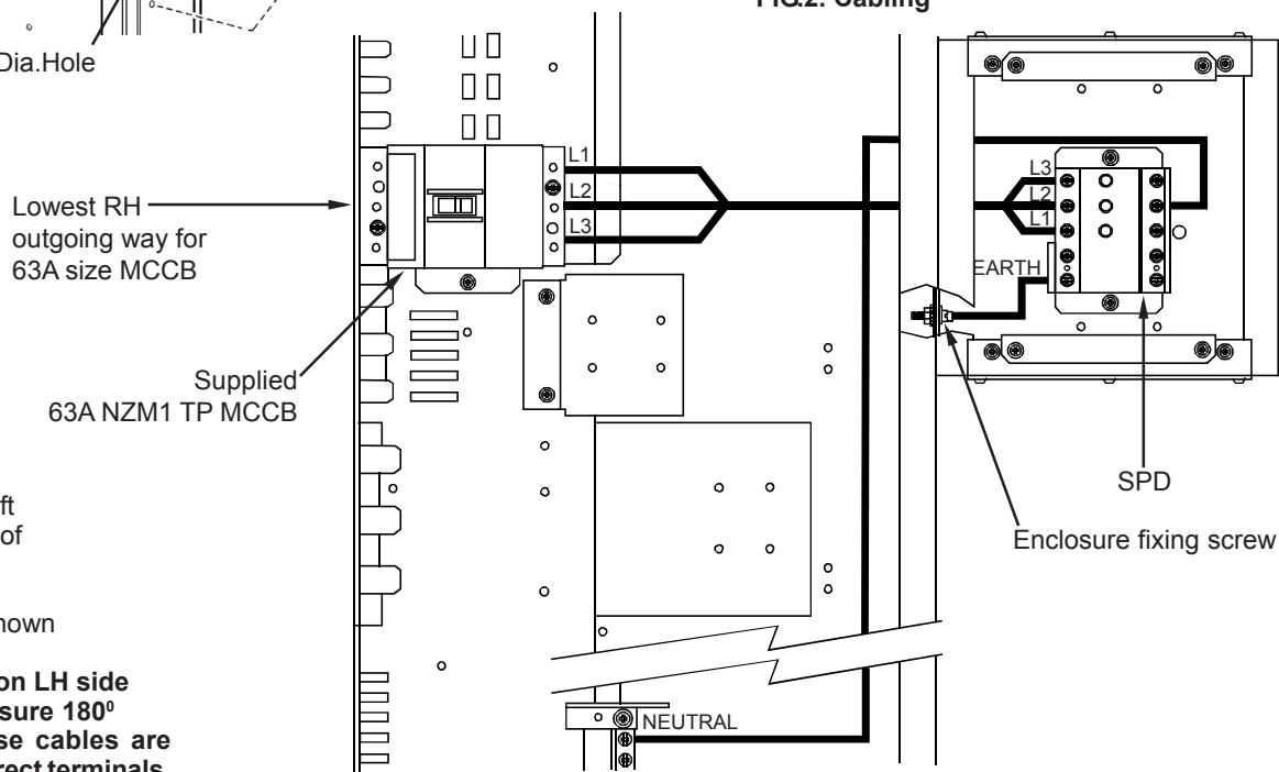
FIG.2. Cabling
