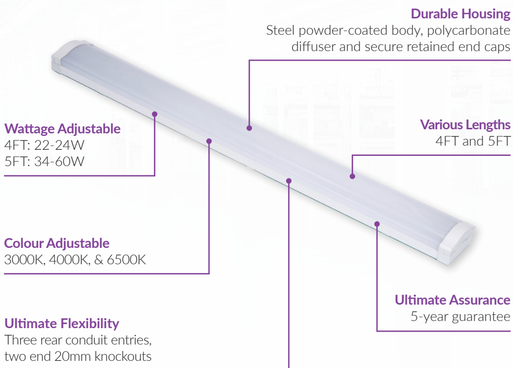
High Power CCT & Wattage Adjustable LED Batten
