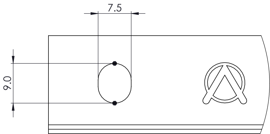
DETAIL A SCALE 2 : 1
