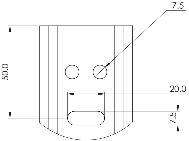
DETAIL A SCALE 1 : 1
