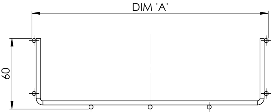
'PROFILE' DETAIL A SCALE 1 : 2
