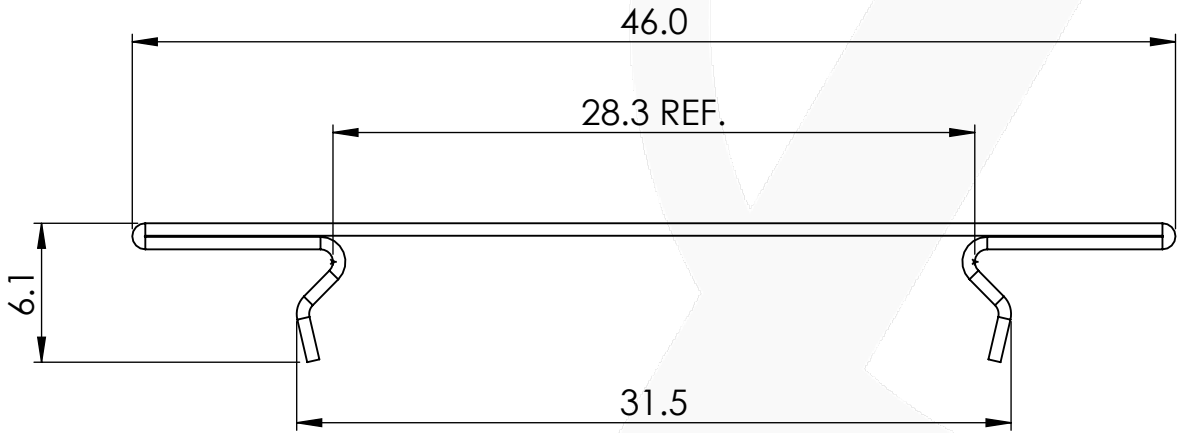
'PROFILE' DETAIL A SCALE 3 : 1
