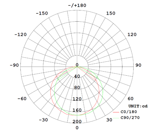
Diagram for RVA48402050 in 4000K. Other diagrams available on request
