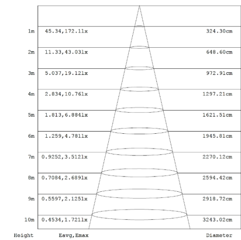
Diagram for RVA48402050 in 4000K. Other diagrams available on request
