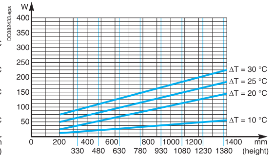
IP43 wall-mounted enclosure
