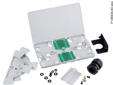
Fusion splice tray kit
