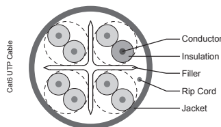
2D4P6PVC3B_Cat6 UTP ACT4P6UCM3RBxx ACT4P6UCR3RBxx ACT4P6ULS3RBxx
