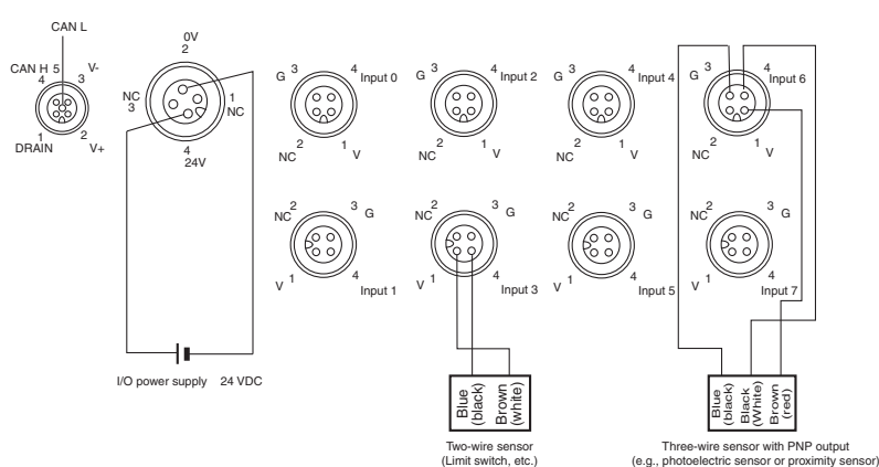
DRT2-ID08CL-1 (PNP)
