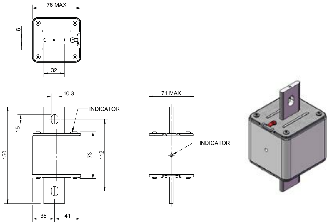
Dimensions (mm) NH3 Blade with bolt holes
