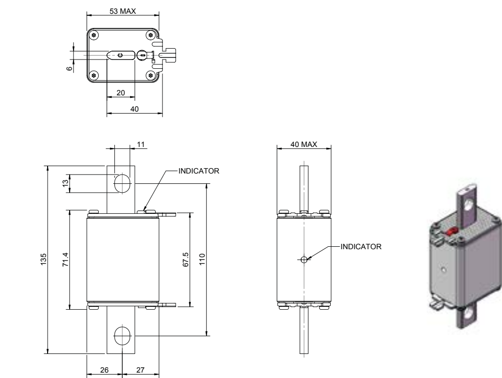
Dimensions (mm) NH1 Blade with bolt holes and lugs
