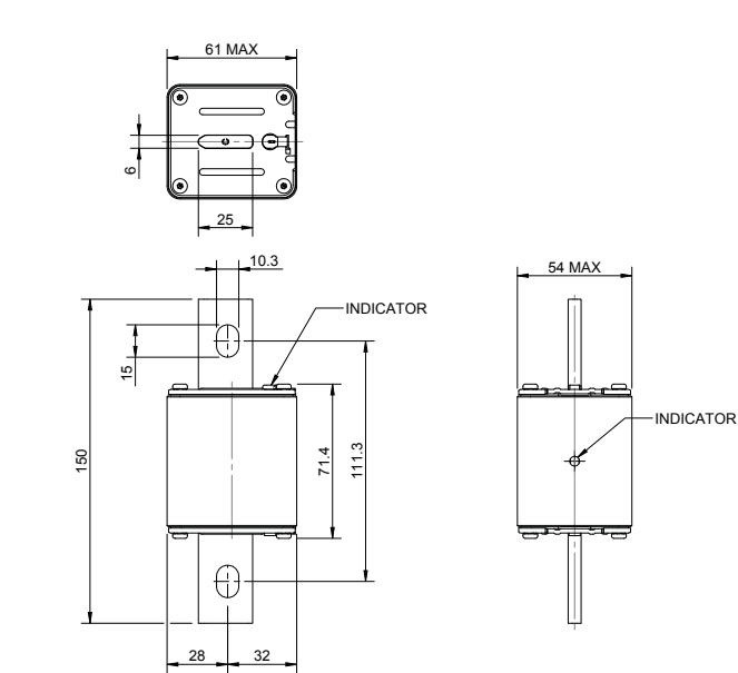
Dimensions (mm), NH2 Bolt holes no lugs
