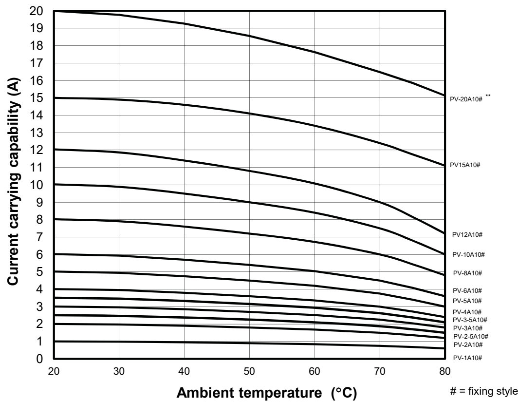
Temperature derating
