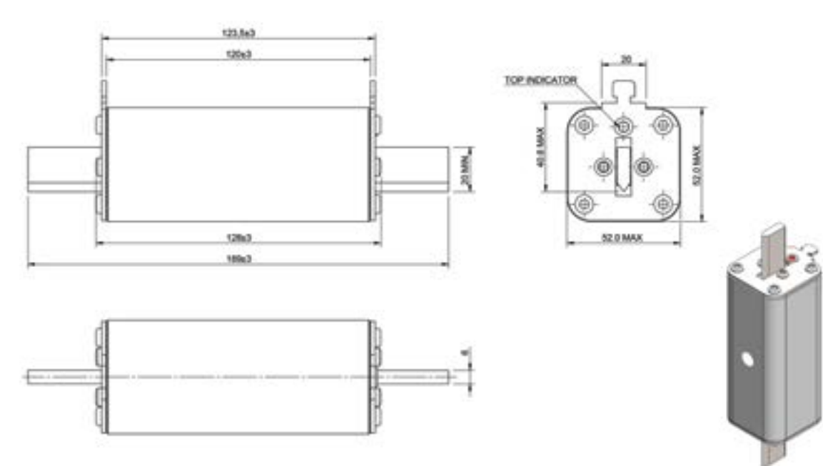
Dimensions (mm) - size 1 Bladed
