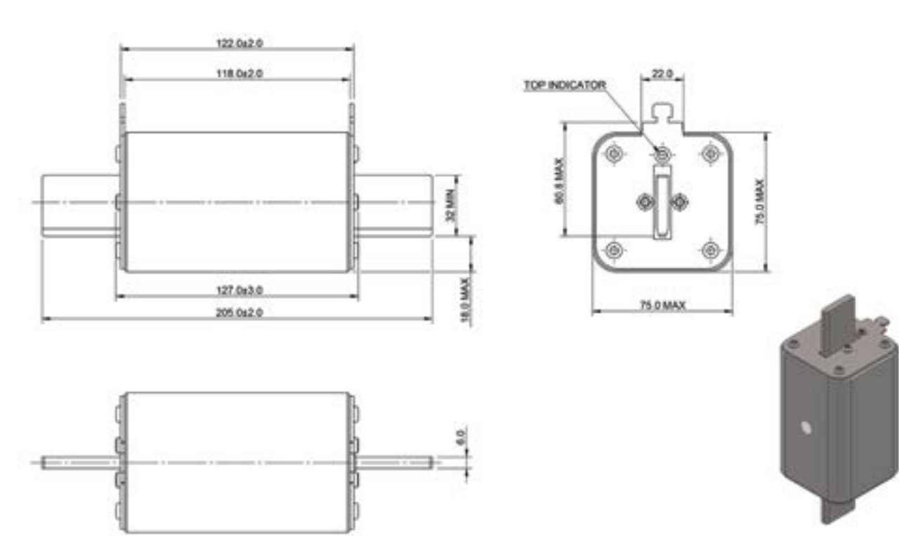
Dimensions (mm) - size 3 Bladed
