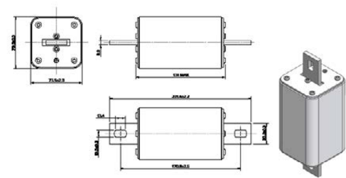
Dimensions (mm) - size 3L Bolted without side indicator
