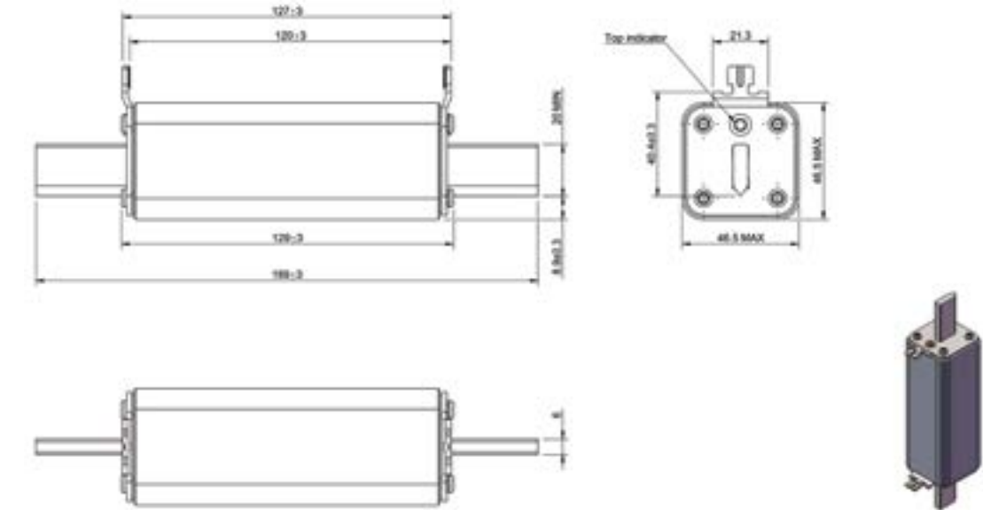
Dimensions (mm)- size 01 Bladed
