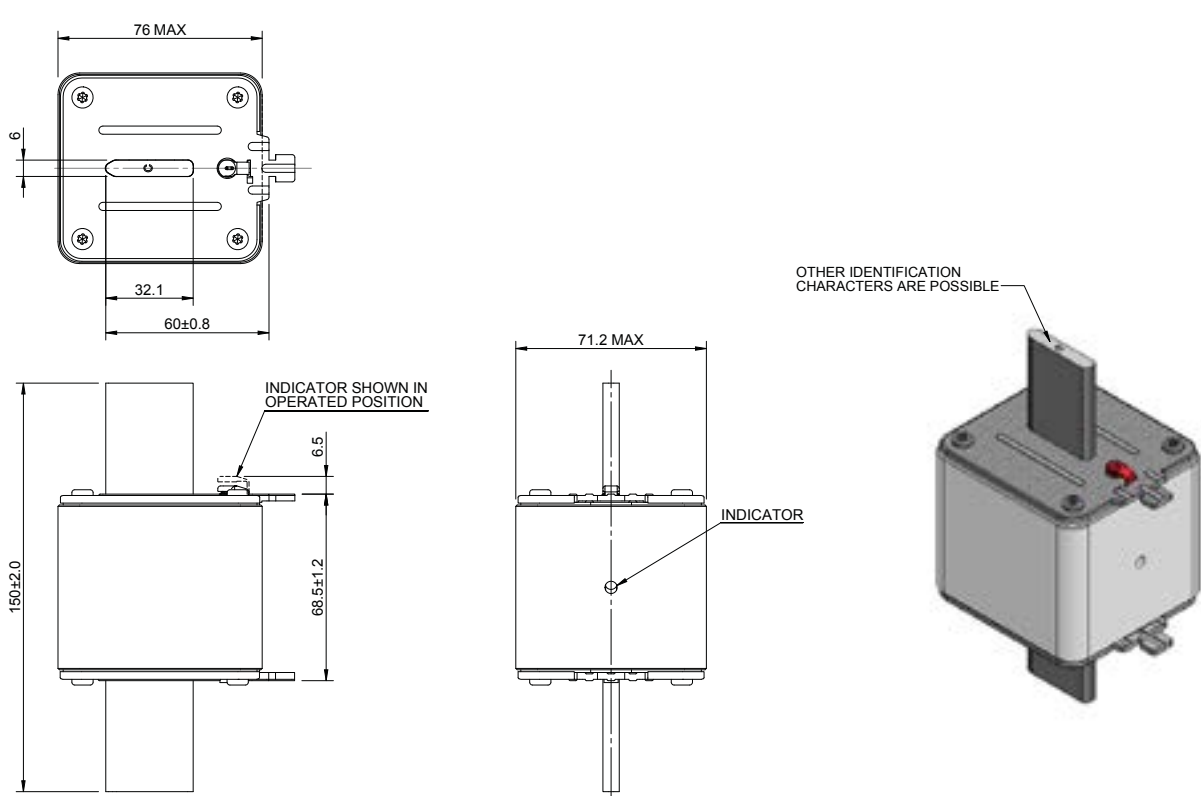
Dimensions (mm) NH3 Blade without bolt holes
