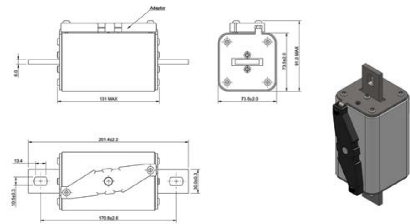
Dimensions (mm) - size 3 Bolted
