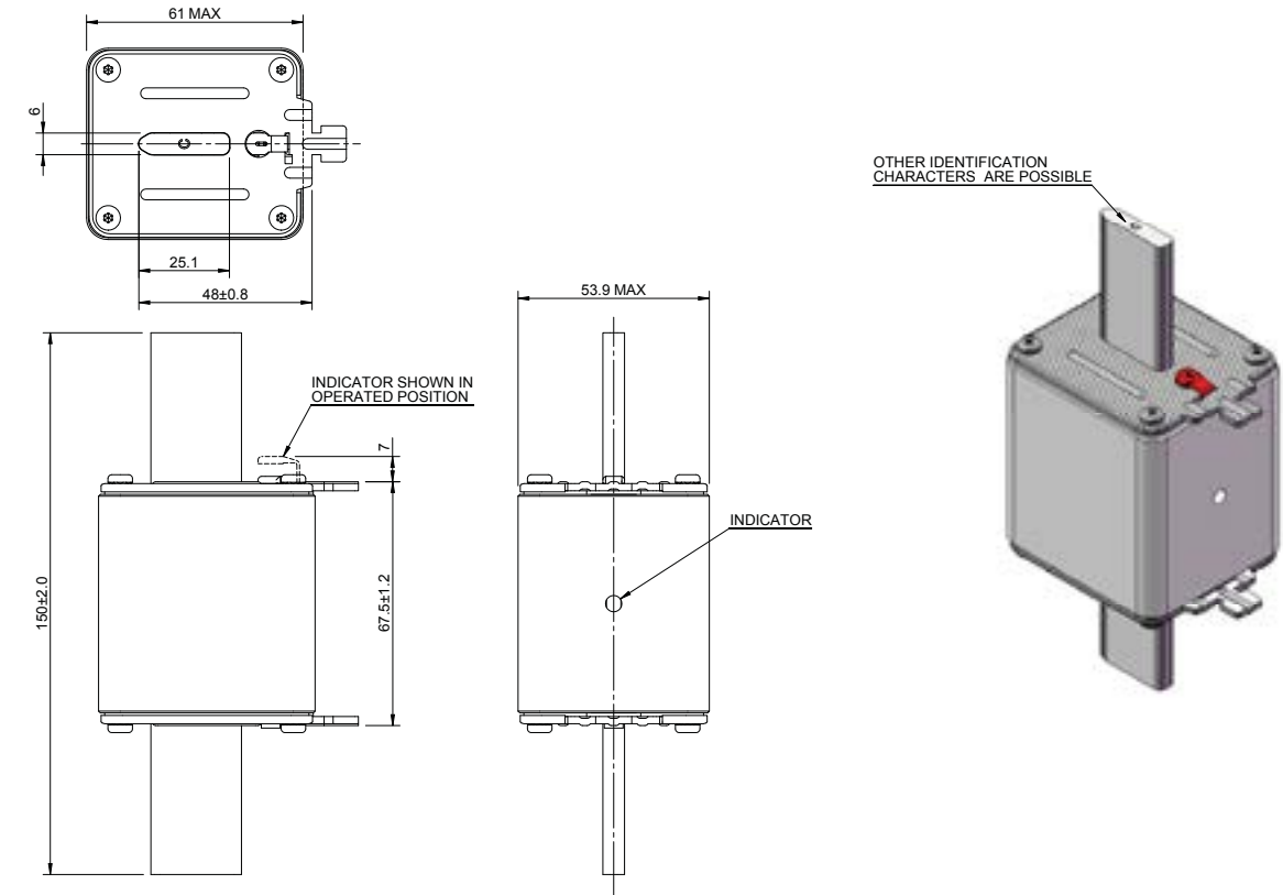
Dimensions (mm) NH2 Blade without bolt holes
