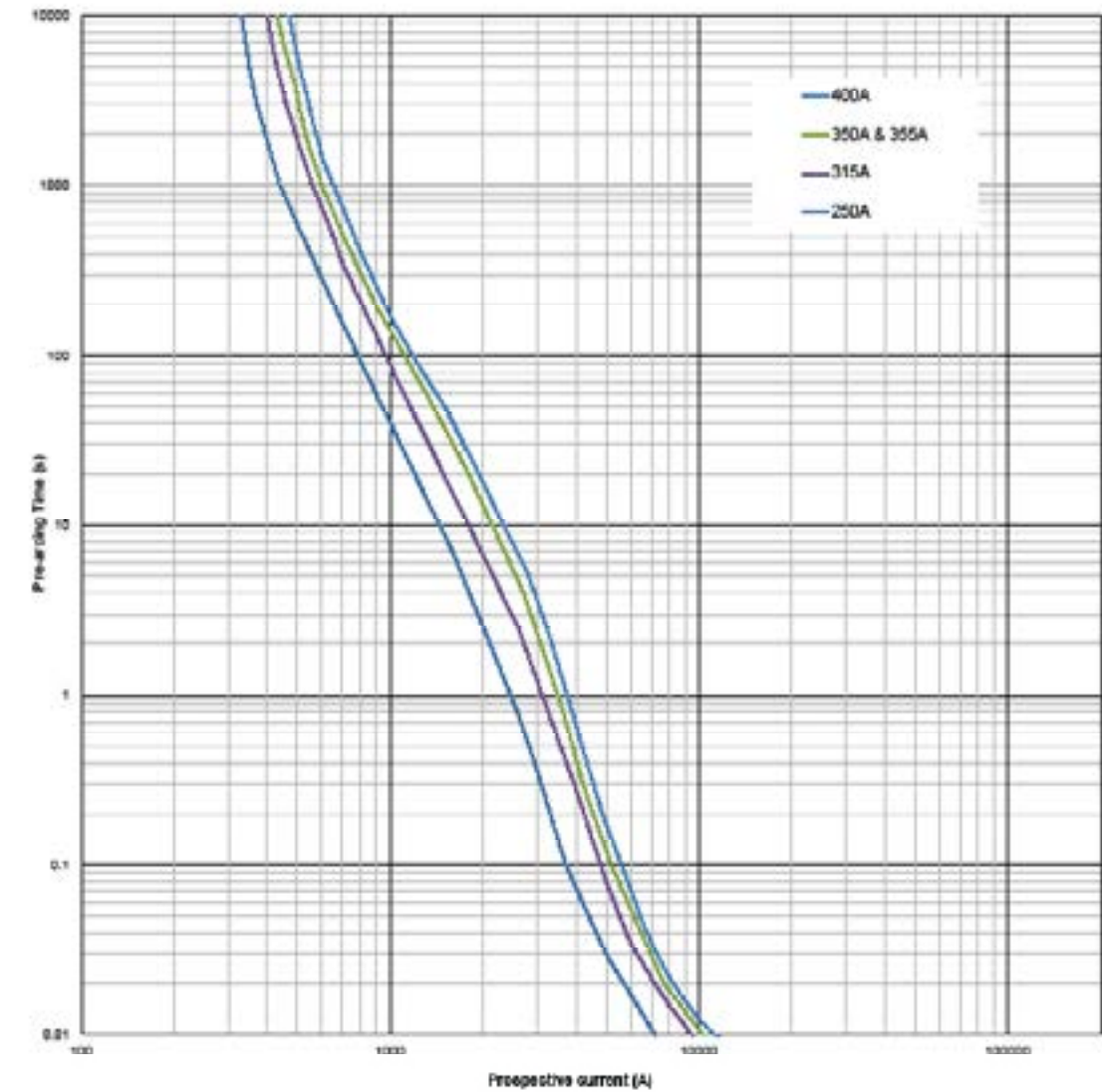
Time current curve
