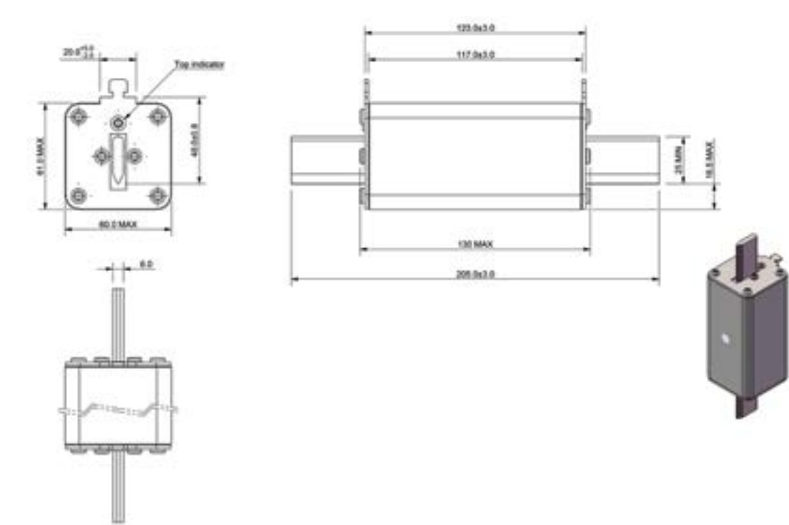
Dimensions (mm) - size 2 Bladed
