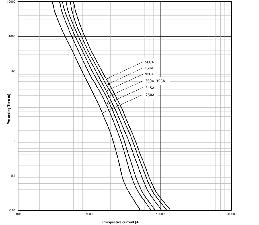
Time-current curve - 1500 V d.c. - 3L - Bladed and bolted - 250 A to 500 A
