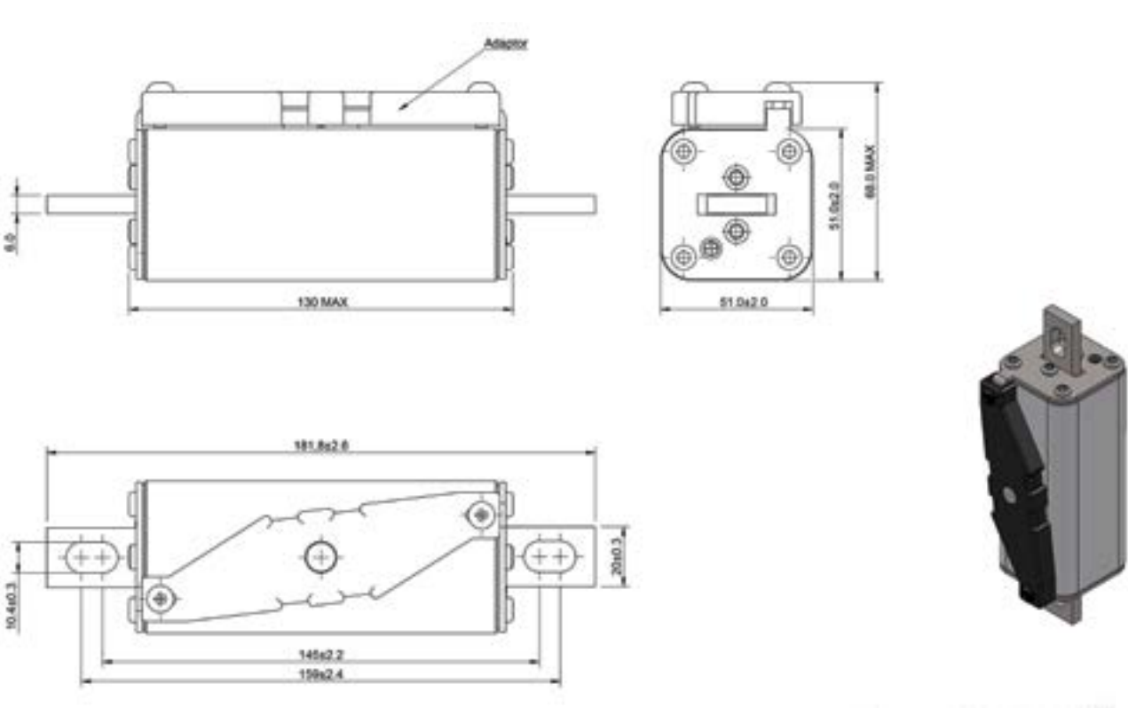
Dimensions (mm) - size 1 Bolted
