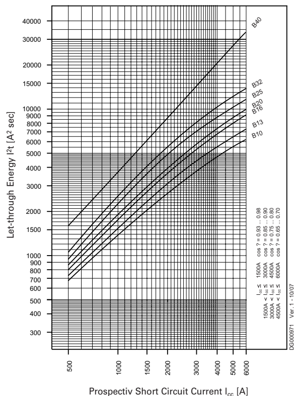
Let-through Energy FRBm6, Characteristic B, 2polig
