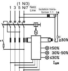
③ Signalisation with Isolation Transformer 1:1 (IEC/EN 60664)
