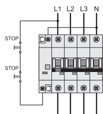
Connection Example Release
