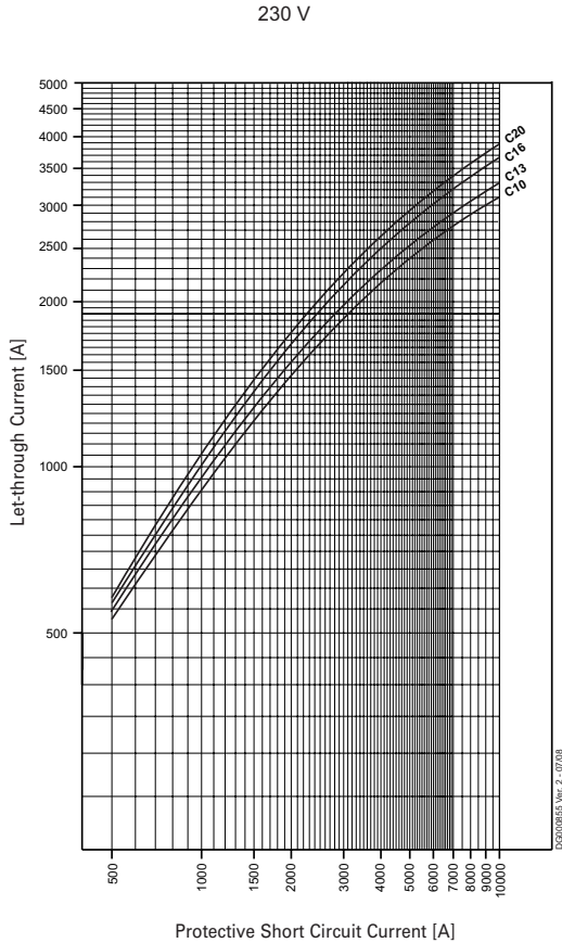
Characteristic C
