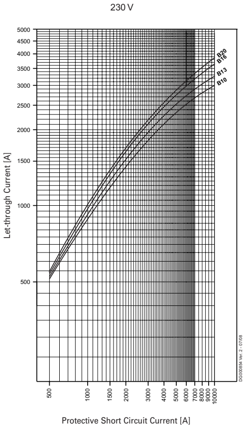
Characteristic B
