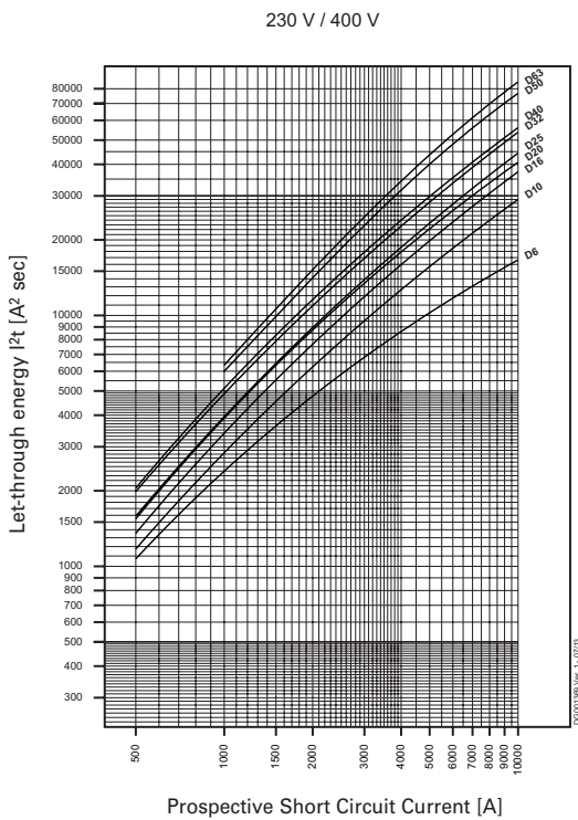
Let-through energy FAZ6, Characteristic D, 1-pole
