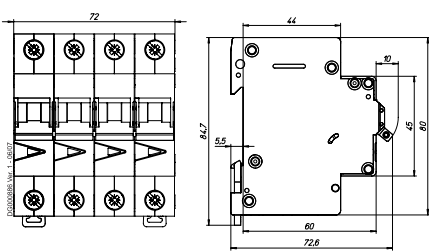
3+N-poles, 4-poles
