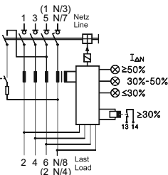
① Basic diagram
