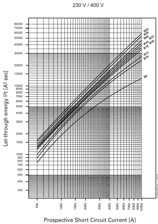
Let-through energy FAZ6, Characteristic B, 1-pole
