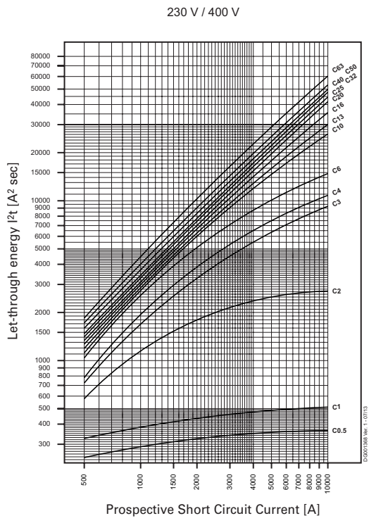
Let-through energy FAZ6, Characteristic C, 1-pole
