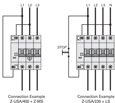
Connection Example 400V and 230V
