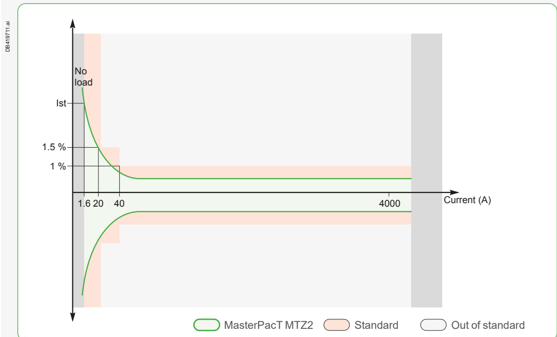
Example: graph for MasterPacT MTZ2
