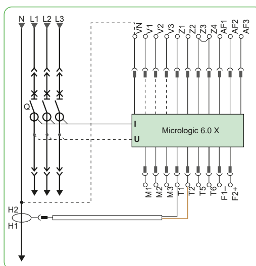
External sensor for neutral and residual earth fault protection (TCE)
