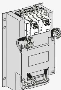
Mounting on the ACP control plate
