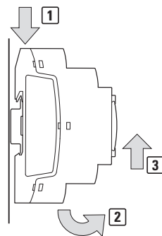
Abb. 16: Demontage
