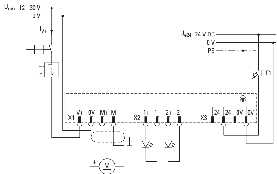
Figure 142: Diagram version 2: Wiring example for XN-322-1DCD-B35
