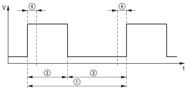
Figure 172: Signal Pulse width modulation
