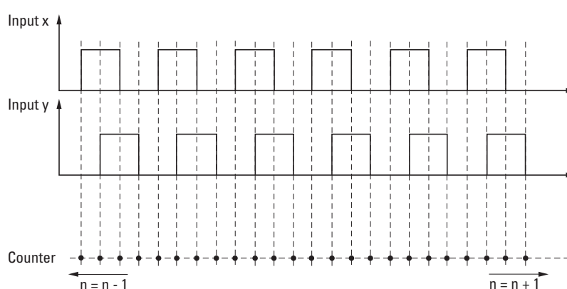
Figure 41: Timing diagram showing how the signals at the XN-322-20DI-PCNT module's inputs are used for counting when using AB quadrature mode with X4 encoding
