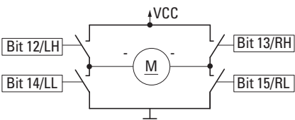
Figure 147: Block diagram showing open motor
