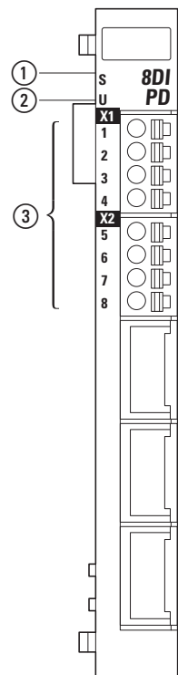
Figure 25: LED signals and pin assignment for XN-322-8DI-PD
