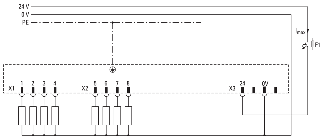
Figure 59: Wiring example
