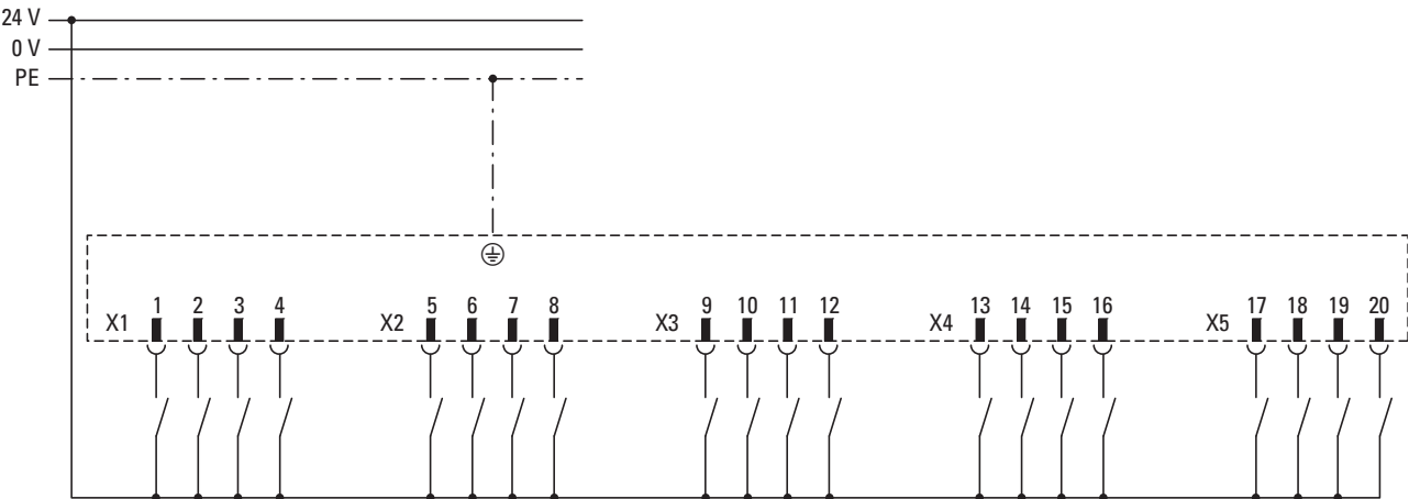
Figure 40: Input wiring
