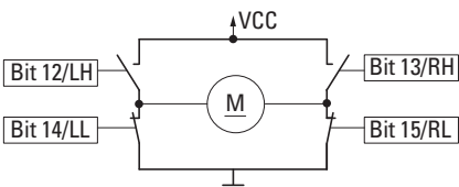
Figure 146: Block diagram showing a motor armature short-circuit
