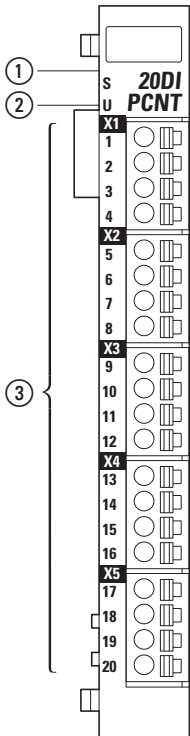
Figure 38: LED signals and pin assignment
