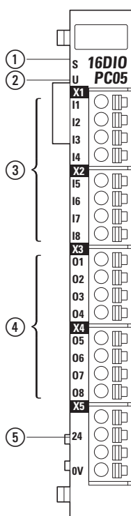
Figure 79: XN-322-16DIO-PC05 LEDs
