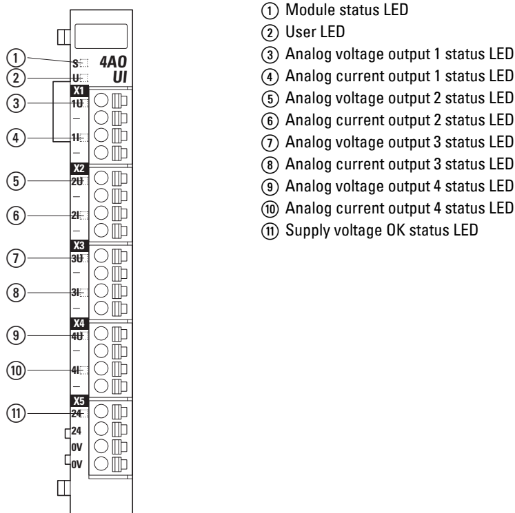
Figure 108: Display
