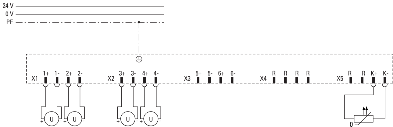
Figure 96: Connecting analog inputs for measuring a sensor at AI1, AI2, AI3, and/or AI4; temperature measurement for KTY10 at X5
