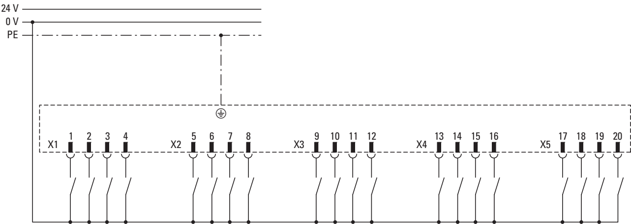
Figure 44: Input wiring
