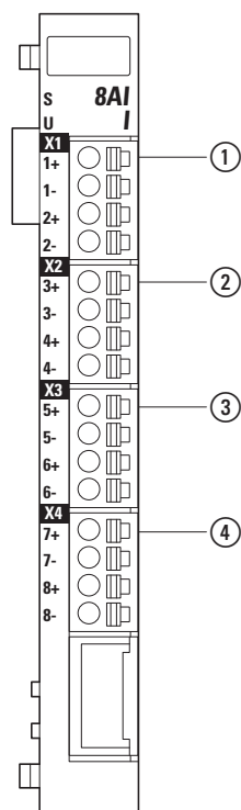
Figure 99: Pin assignment
