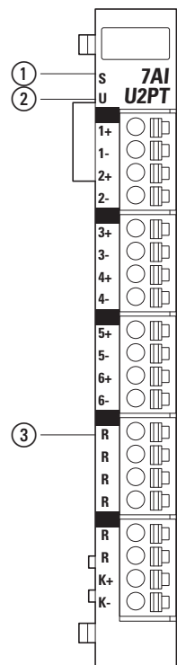
Figure 93: LED signals and pin assignment
