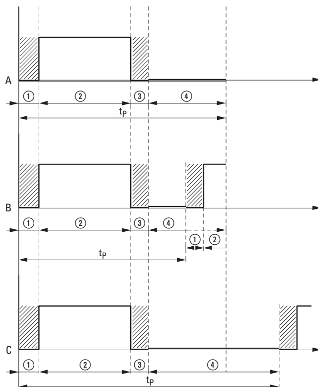
Figure 150: Output signal
