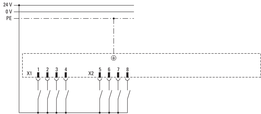
Figure 27: Input wiring
