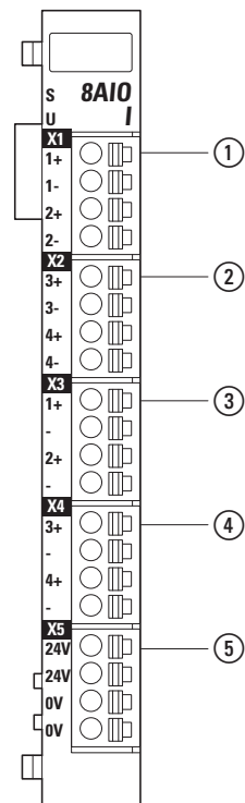
Figure 133: Pin assignment
