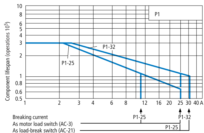
P1 - Characteristic curve
