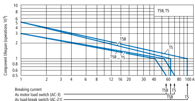
T5, T5B - Characteristic curve
