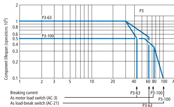
P3 - Characteristic curve
