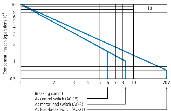
T0 - Characteristic curve
