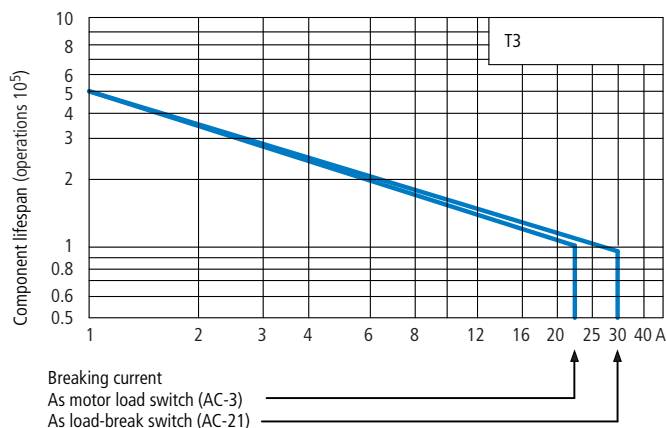
T3 - Characteristic curve
