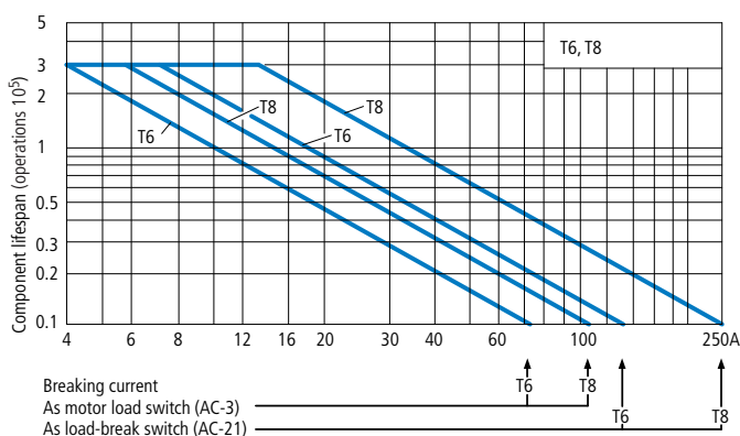
T6, T8 - Characteristic curve
