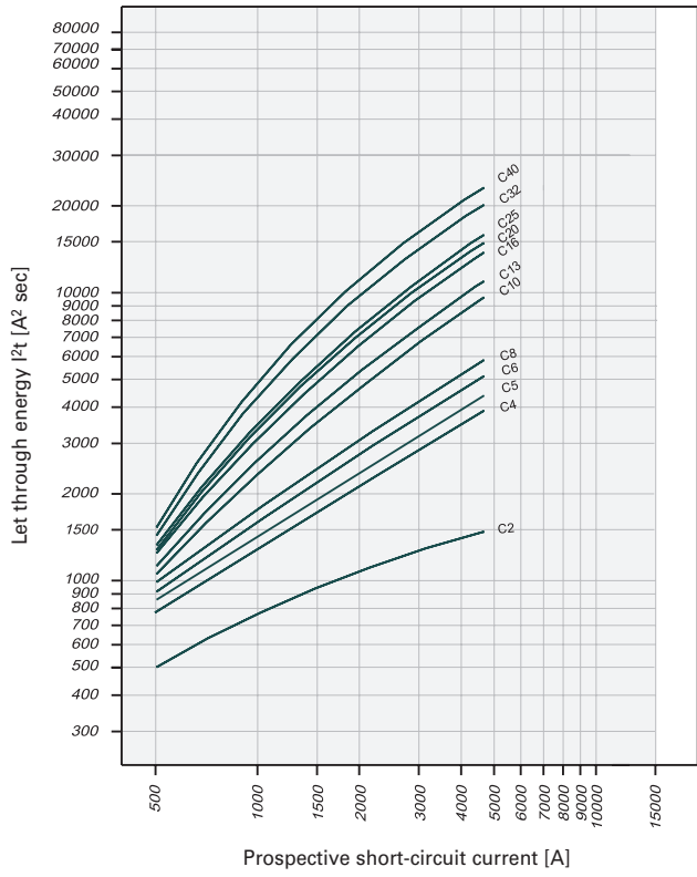
Let-through Energy PKN4, Characteristic C, 1+N-pole
