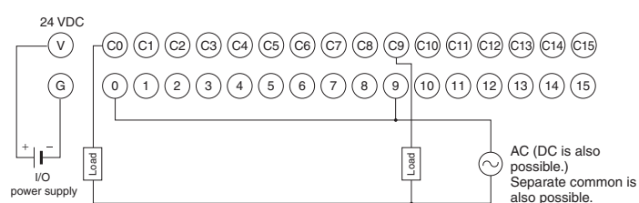
GT1-ROS16
