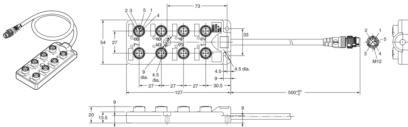
Connections Diagram
