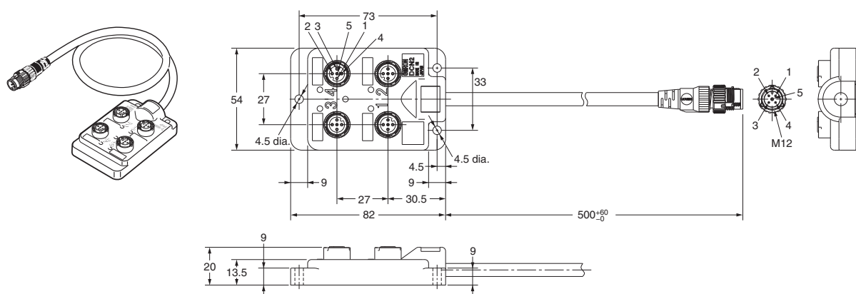
Connections Diagram
