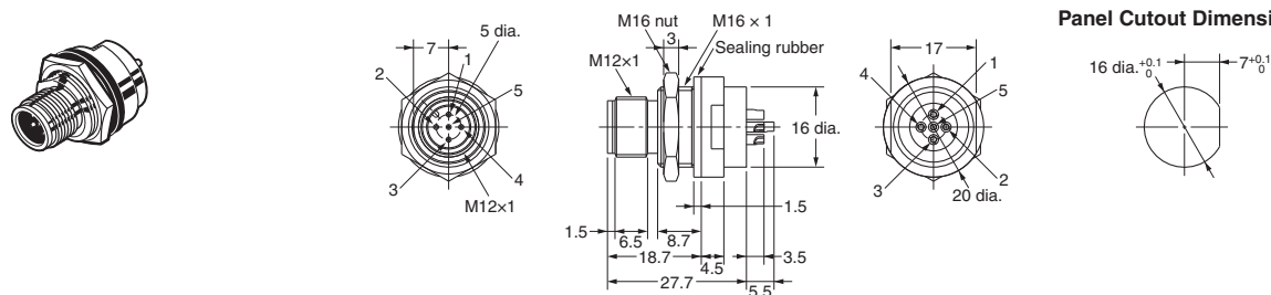
Panel Cutout Dimensions
