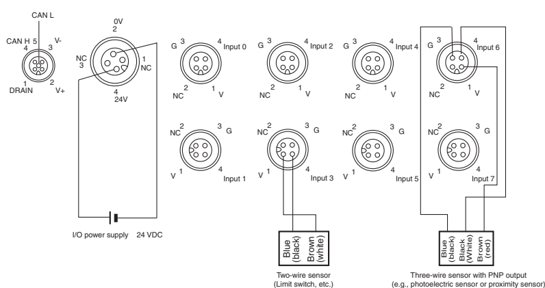
DRT2-ID08CL-1 (PNP)
