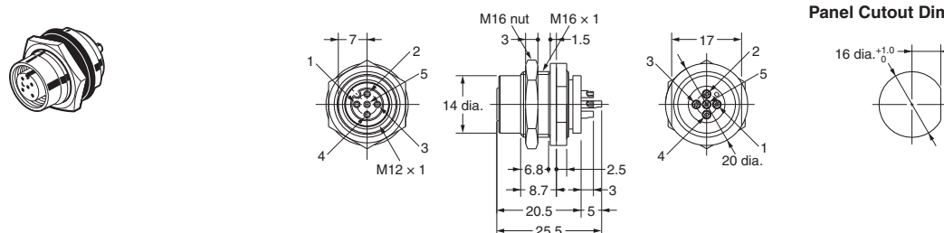
Panel Cutout Dimensions
