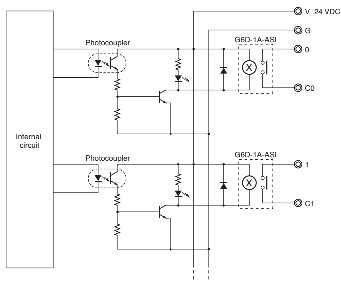
GT1-ROS16
