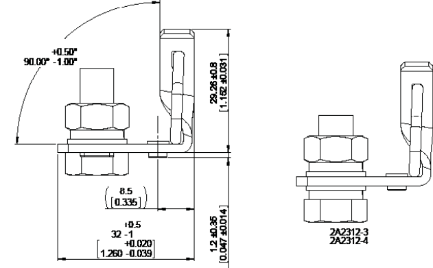
Clinch nut
