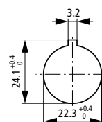
Drilling dimensions
