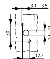
Drilling dimensions
