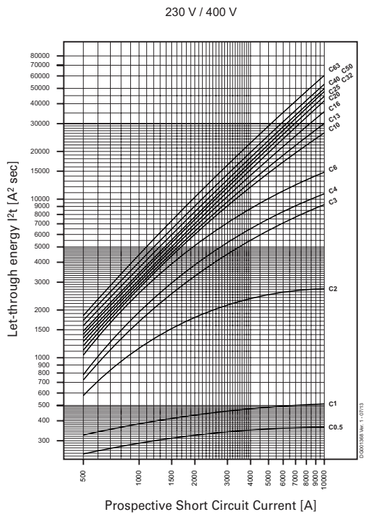
Let-through energy FAZ6, Characteristic C, 1-pole
