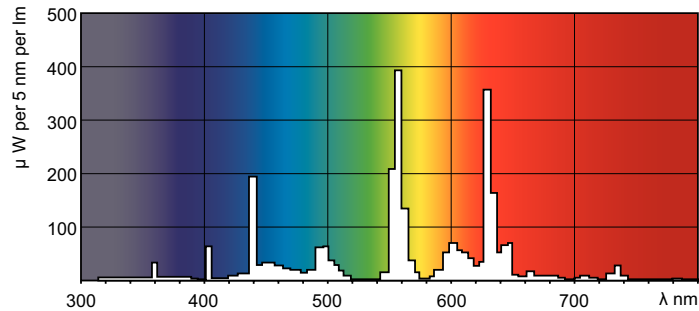
LDPO_TL5HO8SE_840-Spectral power distribution Colour
