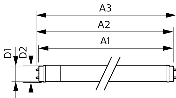
CorePro LEDtube 1500mm 20W 840 T8
