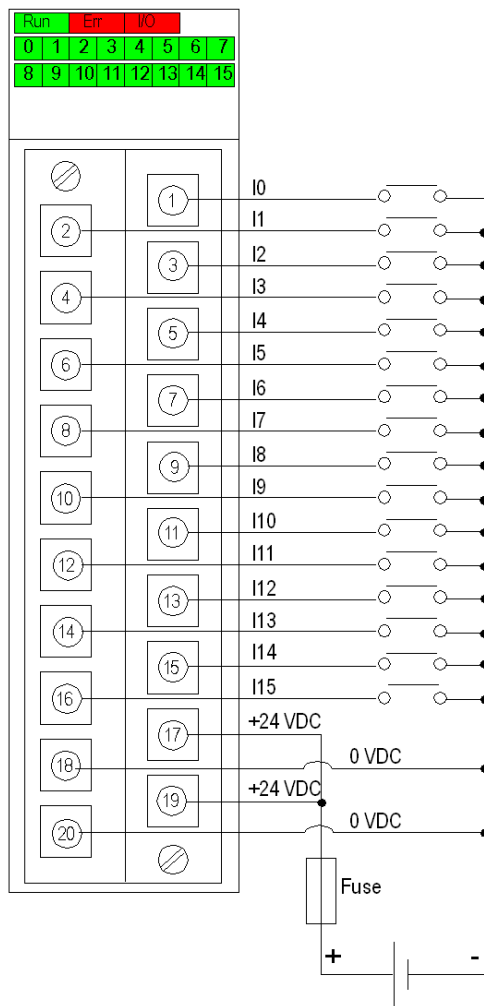
Negative Logic Wiring
