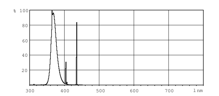
XDPB_XUBTLD_10-Spectral power distribution B/W
