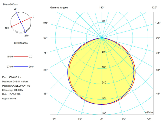
Without reflector - 120 degree
