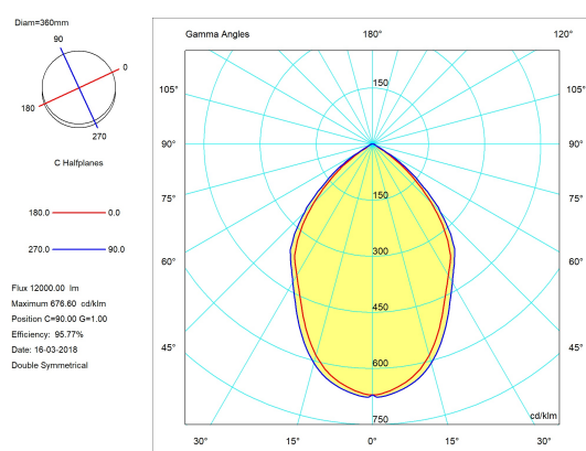
With ACS138 - 90 degree
