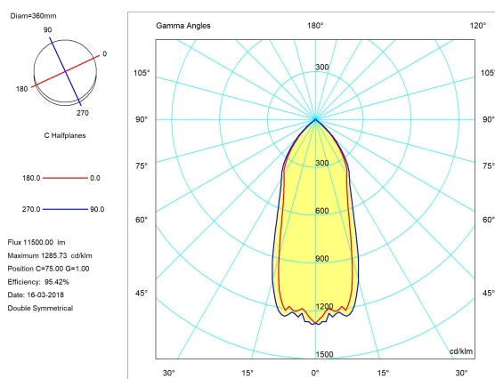
With ACS137 - 60 degree
