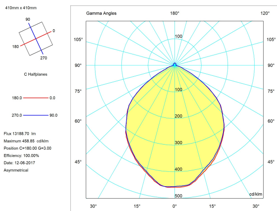
With ACS142 - 90 degree Polycarbonate
