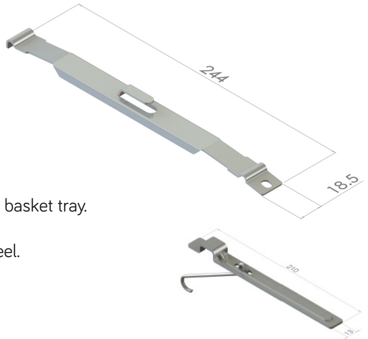
Pulling Tool
