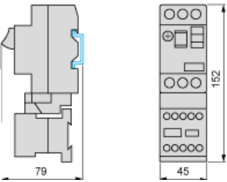
GV2AF3 Combination GV2ME + TeSys d contactor
