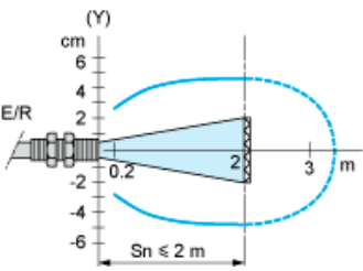
(Y) Ø of beam With reflector XUZC50
