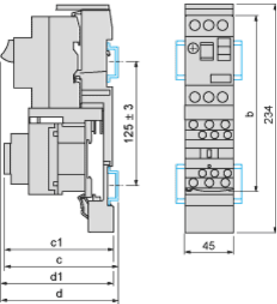
GV2AF4 + LAD311 Combination GV2ME + TeSys d contactor
