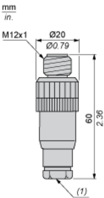
(1) Cable gland : no. 7 plastic (Pg 7)
