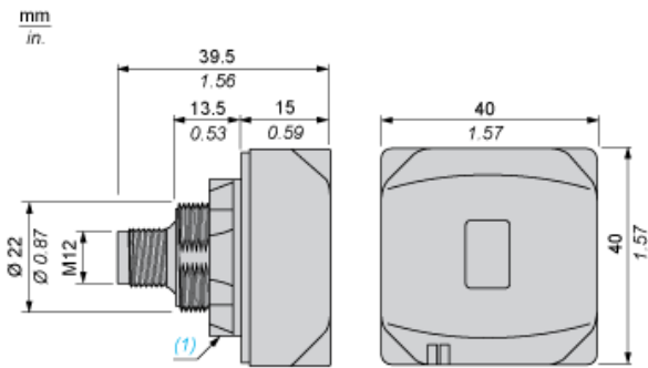
(1) Locking nut
