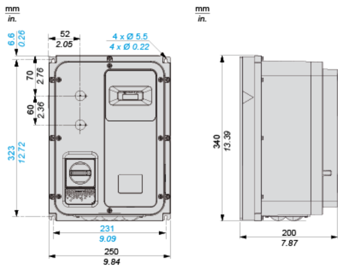
Front and Left View
