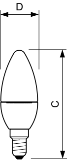
LED ND 4-25W E14 827 220-240V B35 CL
