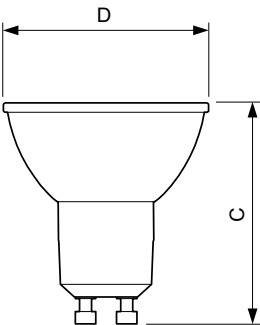
Corepro LEDspot 4.6-50W GU10 840 36D UK
