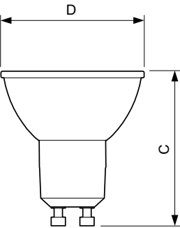
Corepro LEDspot 4.6-50W GU10 865 36D UK
