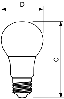
Bulb A60S 230V 5.5-40W 470lm 2700K E27
