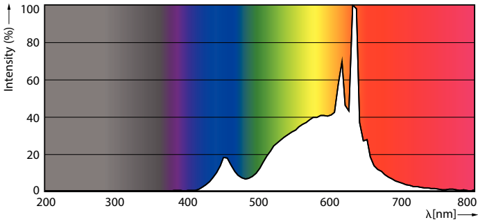
LEDBulb CorePro E27 A60 5W
