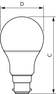
Bulb A60S+ 230V 8.5-60W 806lm 2700K B22
