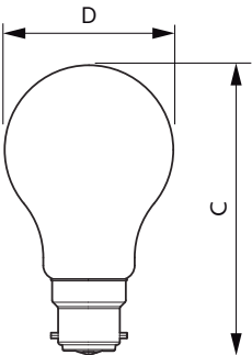
A60 230V 9-60W 806lm 2700-2200K B22 D CL
