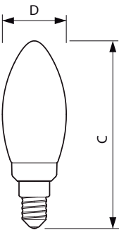
B35 230V 4-25W 250lm 2700-2200K E14 D CL
