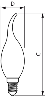
BA35 230V 40W 470lm 2700-2200K E14 D CL
