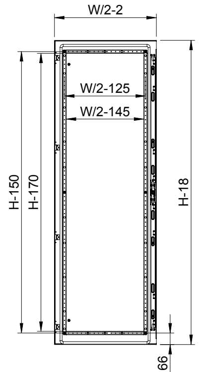
Inside right door view
