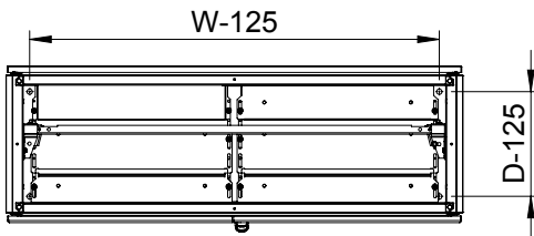
Sectional top view W=1200
