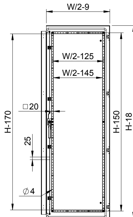
Inside left door view
