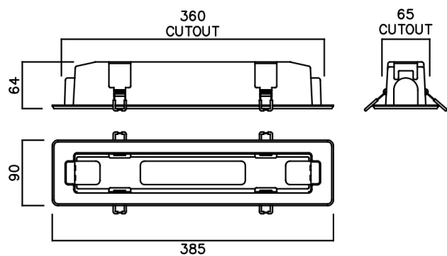
RECESSED MOUNTING KIT (NAL/RMK)
