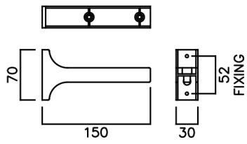
SIDE WALL MOUNTING KIT (NAL/SWMK)
