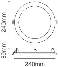
Cut out: Ø220-230mm
